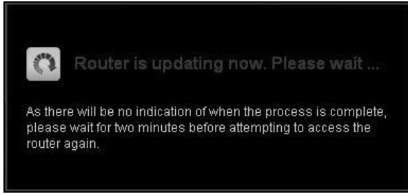
Figure 139 Firmware Uploading
