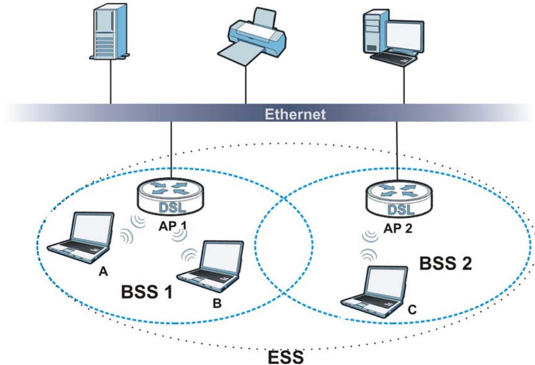
Figure 161 Infrastructure WLAN
