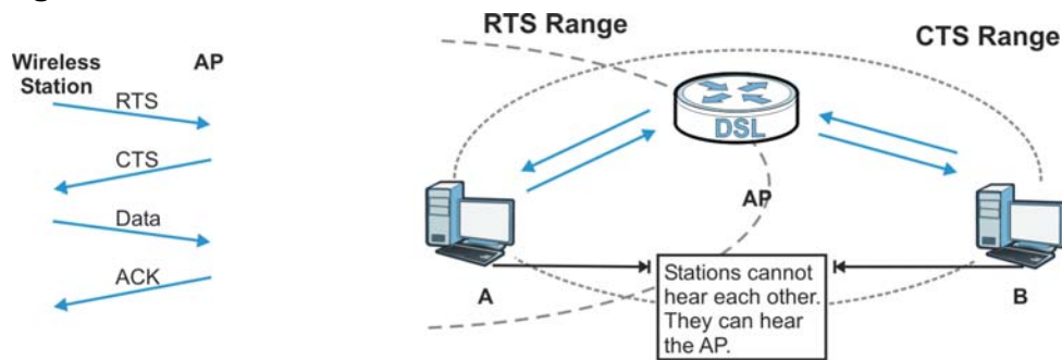
Figure 162 RTS/CTS
