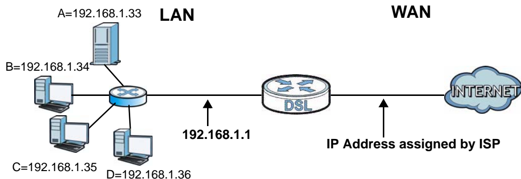
Figure 64 Multiple Servers Behind NAT Example
