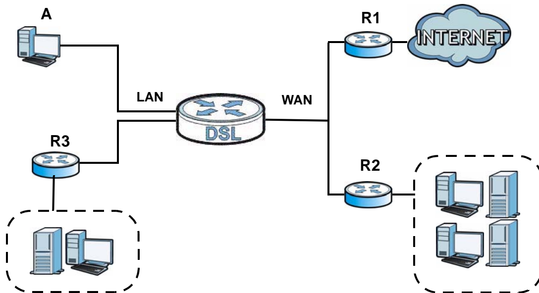
Figure 76 Example of Static Routing Topology
