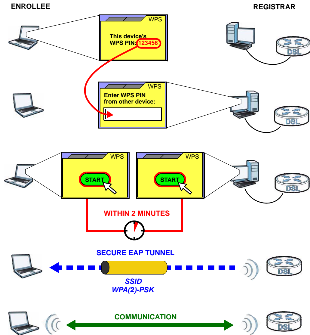
Figure 58 Example WPS Process: PIN Method
