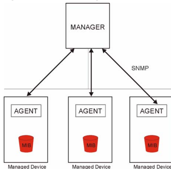
Figure 91 SNMP Management Model
