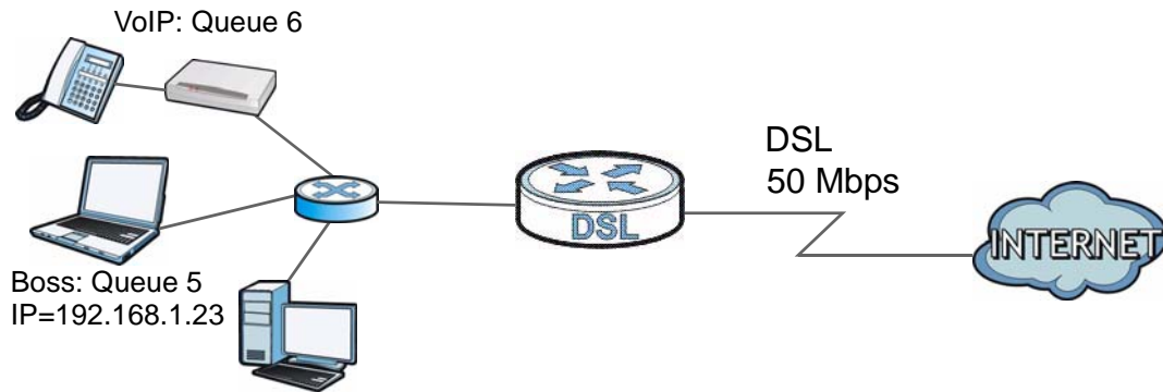
Figure 83 QoS Example
