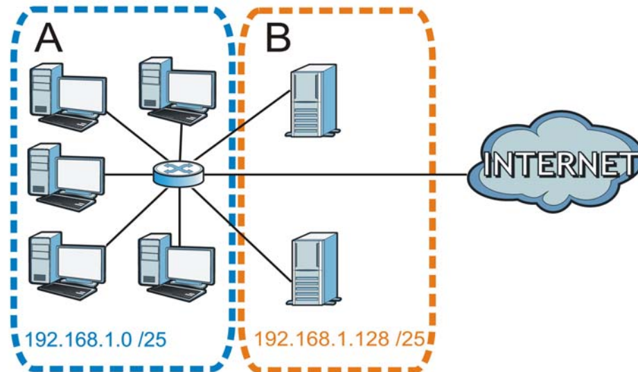
Figure 165 Subnetting Example: After Subnetting
