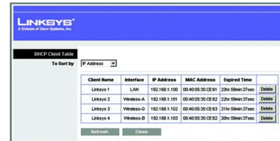
Figure 5-50: Status Tab - Local Network
