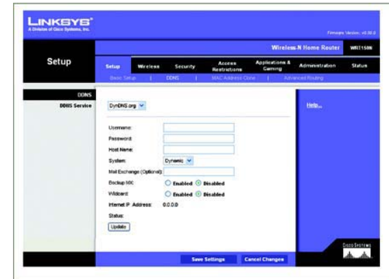
Figure 5-9: Setup Tab - DDNS (DynDNS.org)
