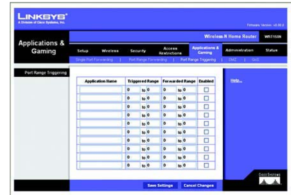
Figure 5-31: Applications & Gaming Tab - Port Range Triggering
