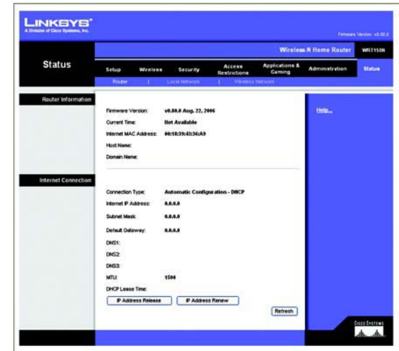
Figure 5-48: Status Tab - Router
