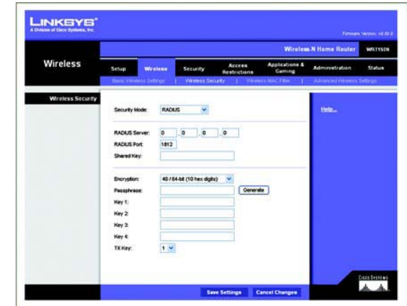
Figure 5-19: Wireless Security - RADIUS
