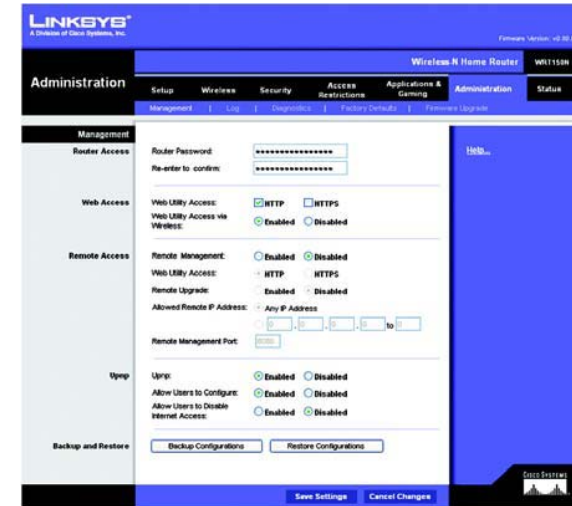
Figure 5-40: Administration Tab - Management
