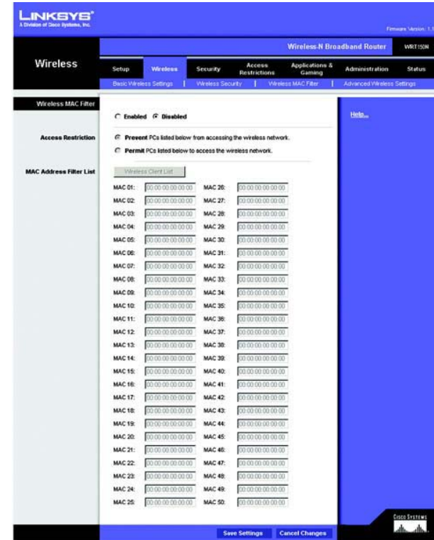
Figure E-4: Wireless MAC Filter
