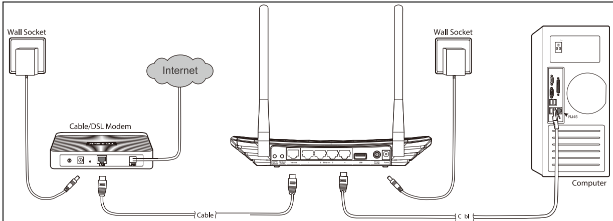
Figure 2-1 Hardware Installation
