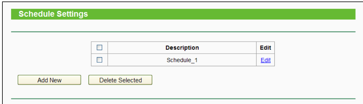
Figure 4-85 Schedule Settings
