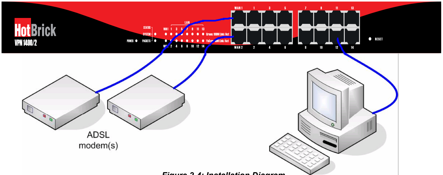
Figure 2-4: Installation Diagram
