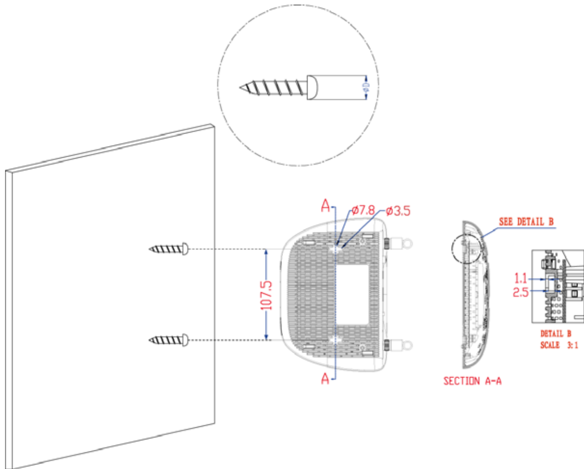
Figure 2-2 Wall-mount Install
