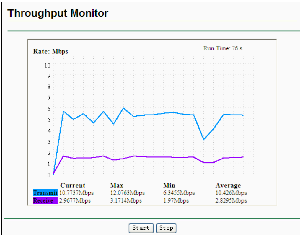
Figure 4-20 Throughput Monitor
