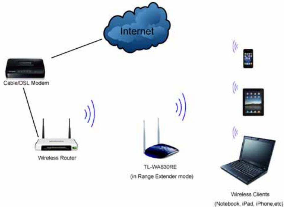
Figure 2-1 Typical connection of TL-WA830RE (in Range Extender mode)
