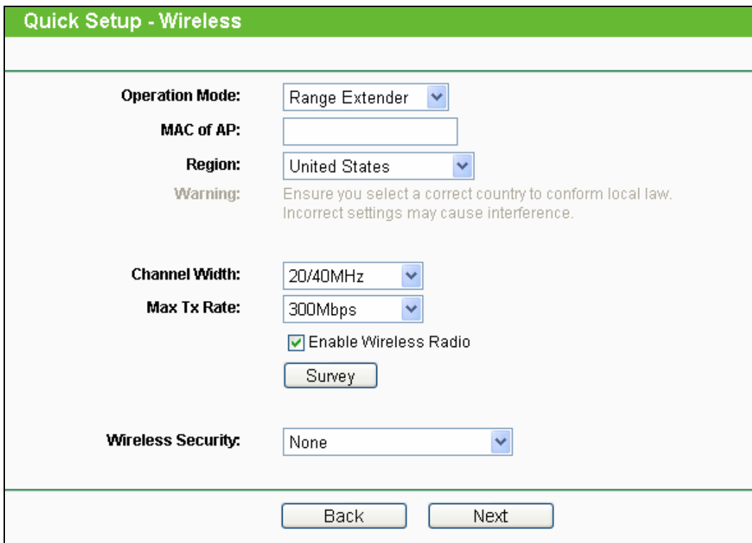
Figure 3-10 Quick Setup - Wireless
