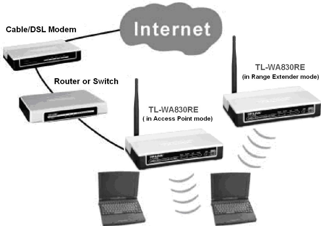
Figure 2-1 The Example of Infrastructure Network Incorporating the TL-WA830RE
