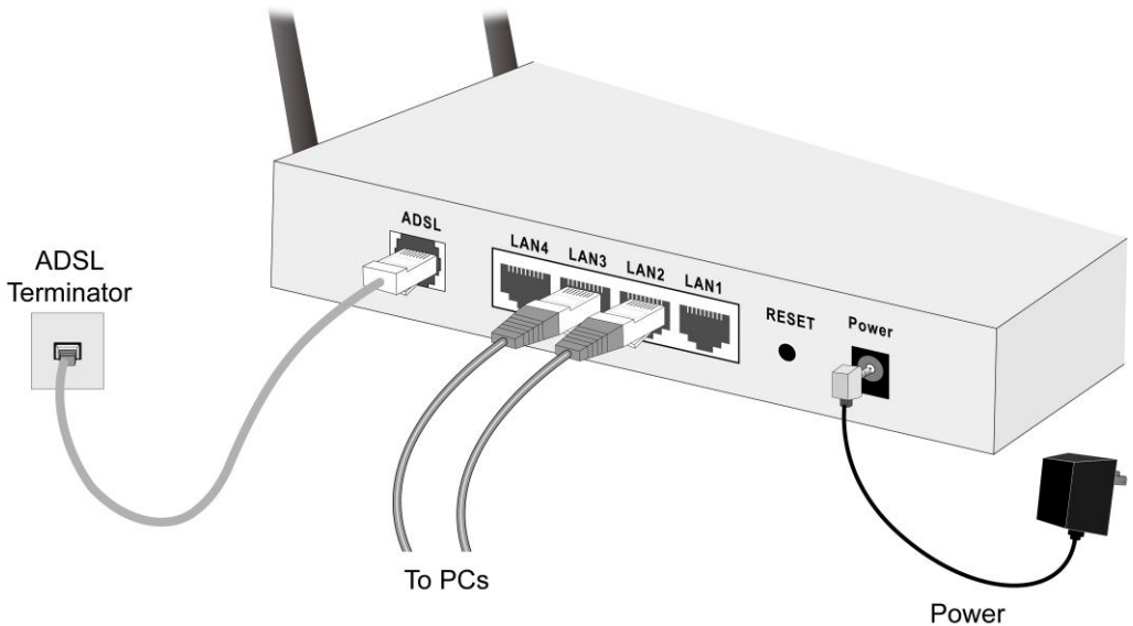
Figure 4: Installation Diagram
