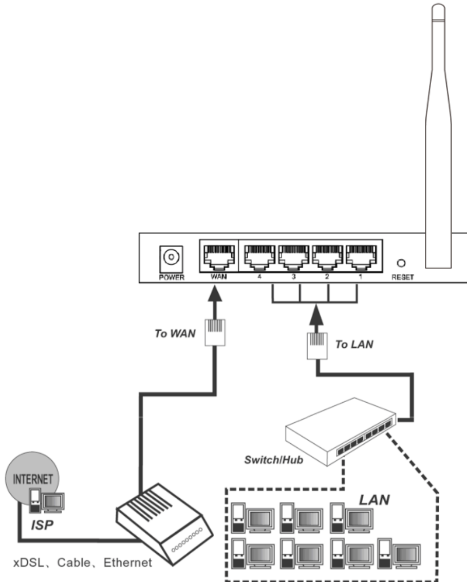
Figure 2-1 Hardware Installation of the RNX-N150RT 150M Wireless Lite-N Router
