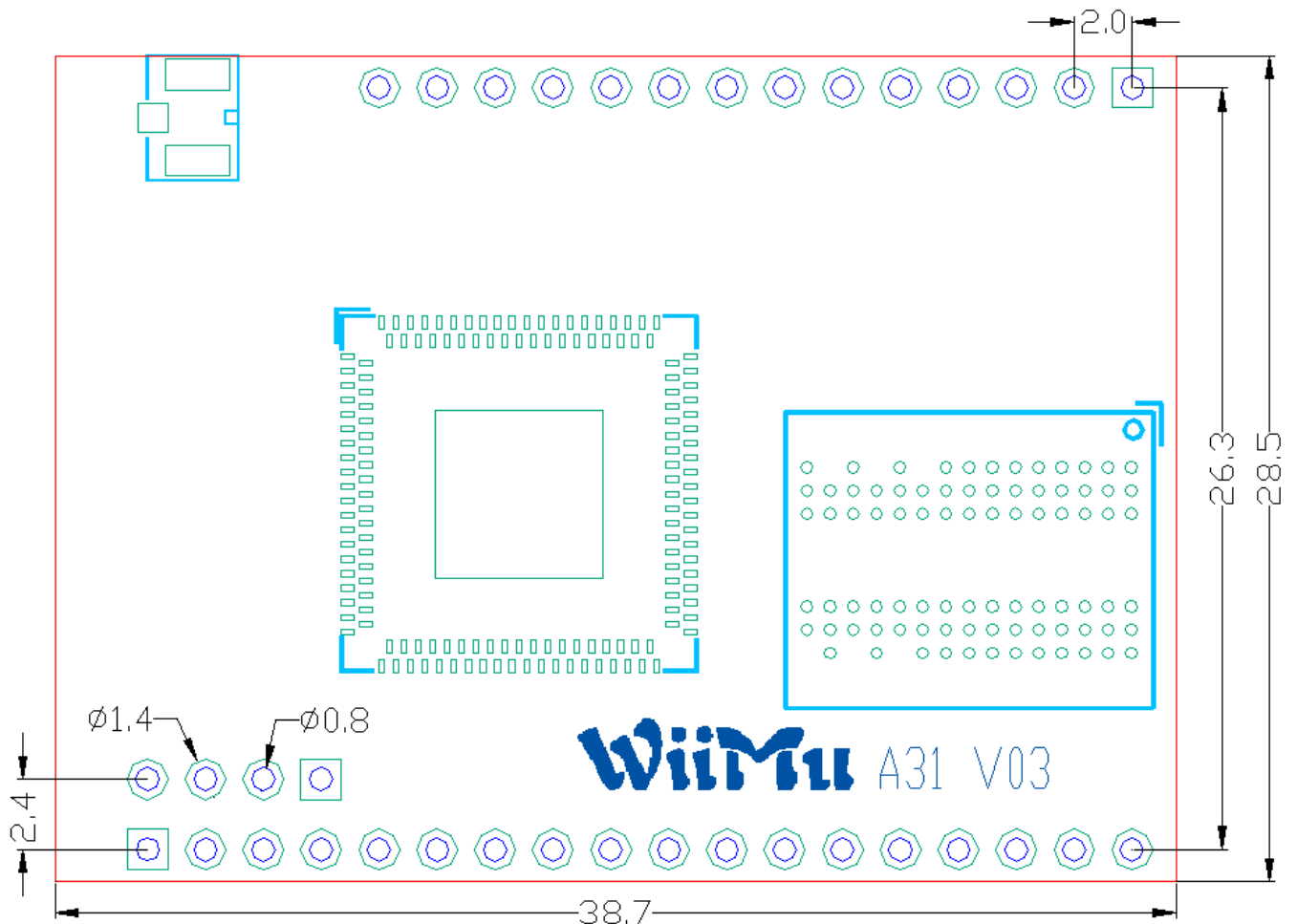
Figure 2-2: LinkPlay A31-2 physical dimension
