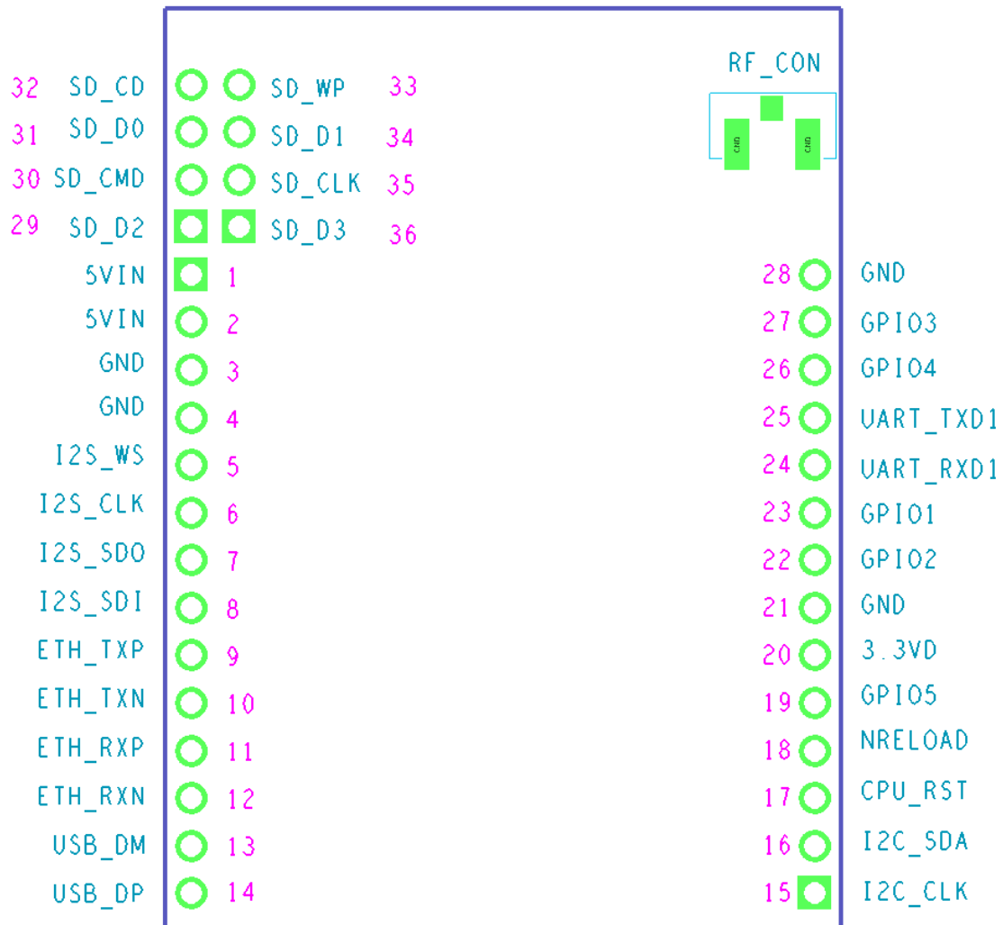
Figure 2-1 A31-2 interface pins
