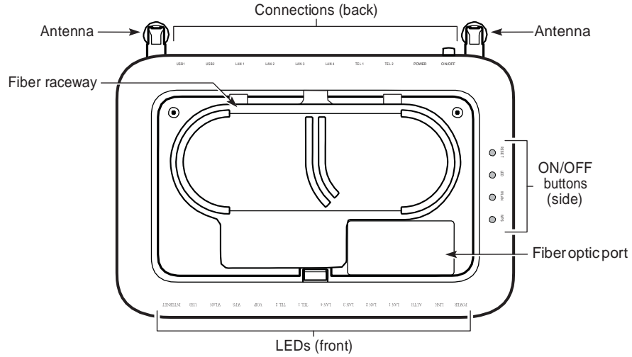
Figure 23 G-240W-F ONT Reset, LED, WLAN, and WPS buttons and fiber optic connection (bottom and side view)
