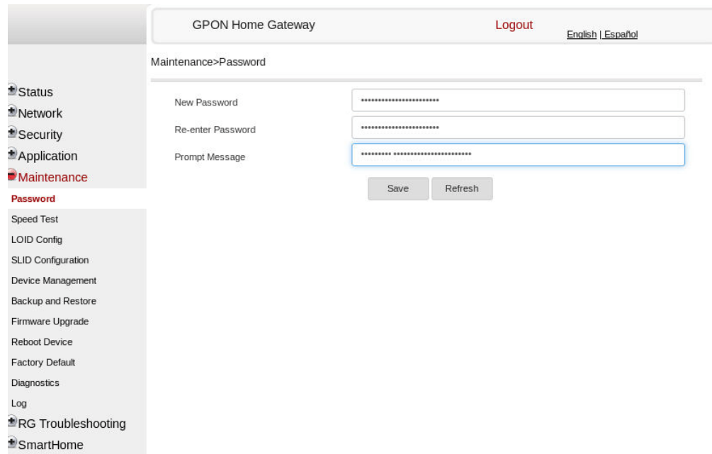
Figure 77 Password window
