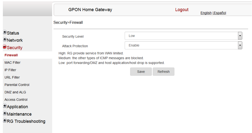
Figure 47 Firewall window
