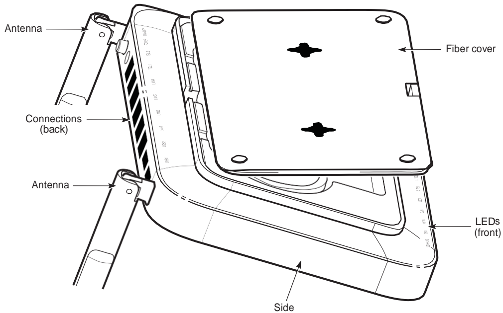
Figure 24 G-240W-F indoor ONT with fiber cover open
