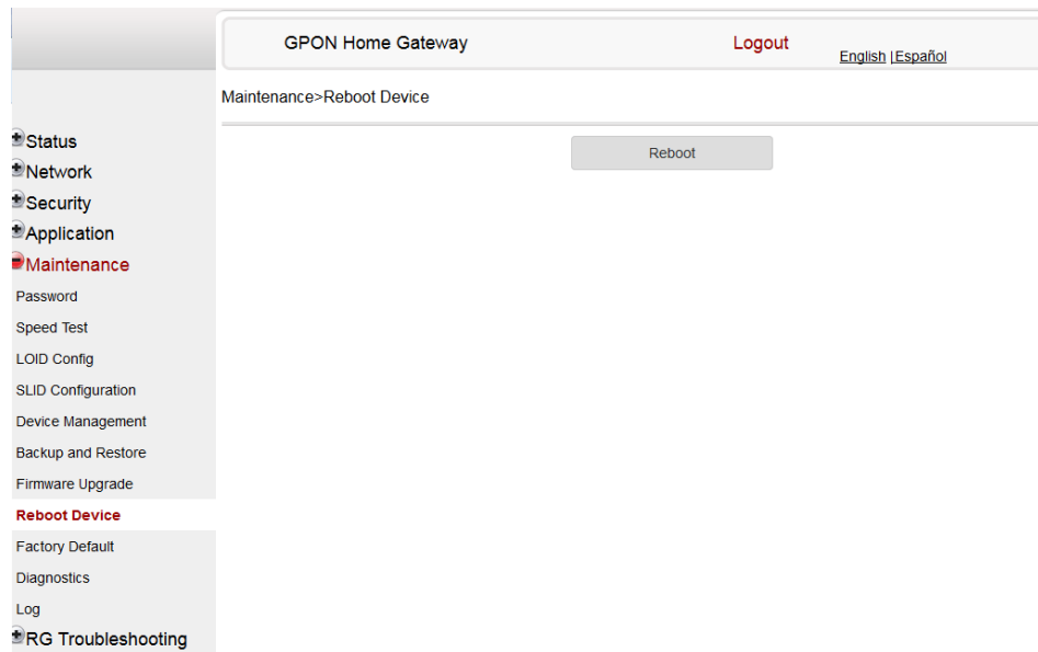
Figure 68 Reboot window
