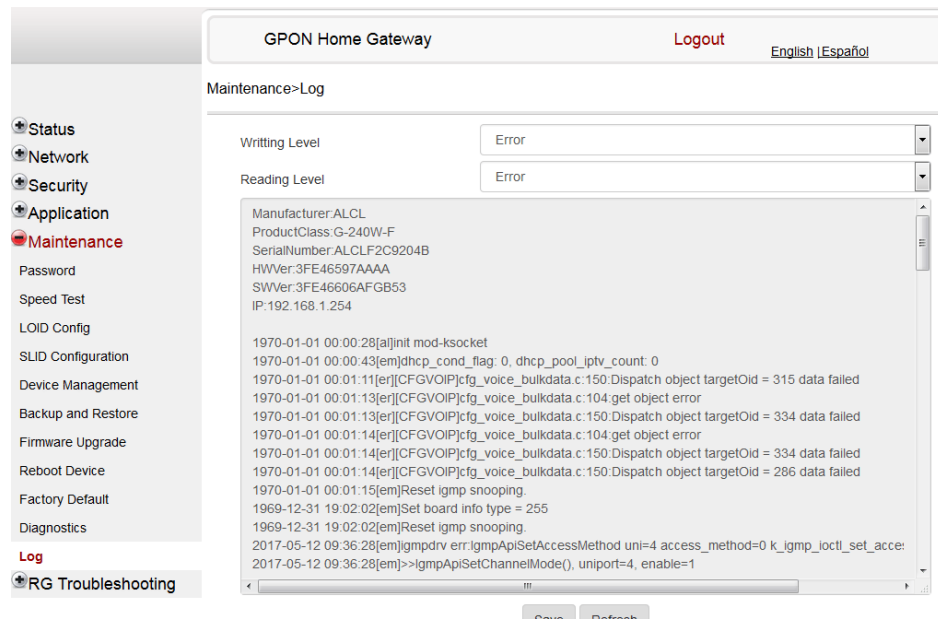
Figure 71 Log window
