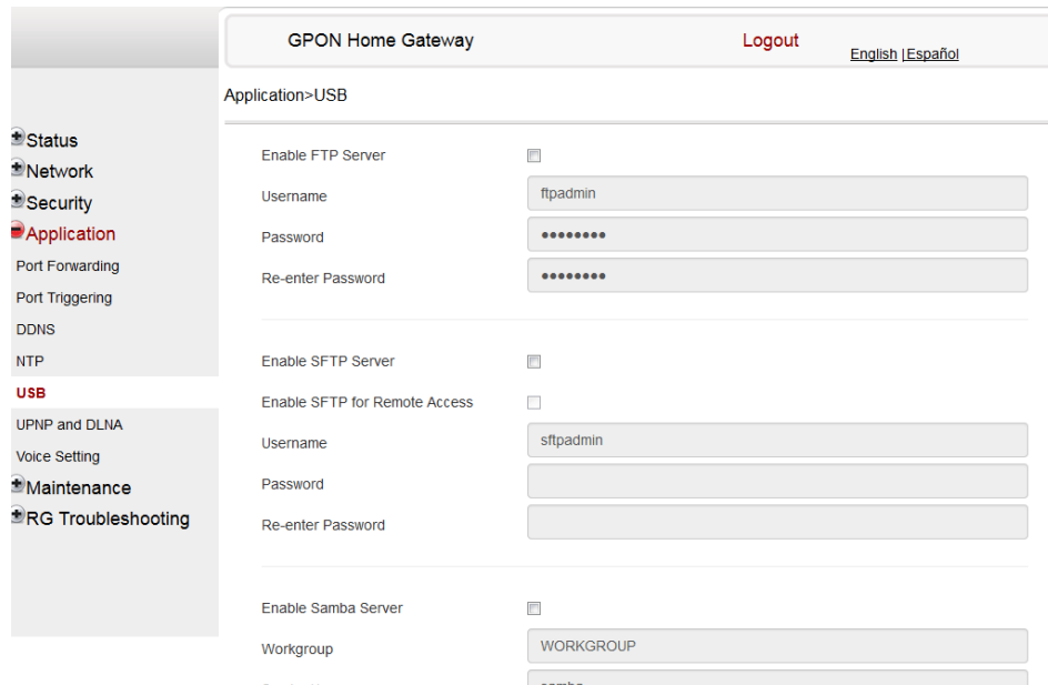
Figure 58 USB window
