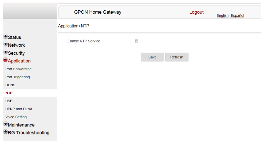
Figure 57 NTP window
