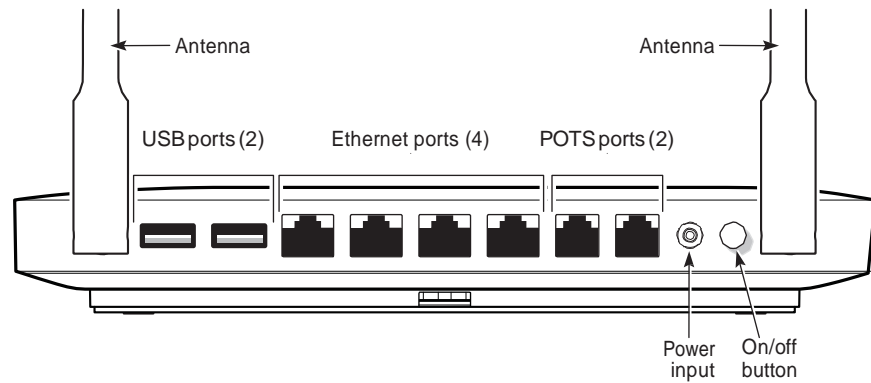
Figure 22 G-240W-F indoor ONT connections (back view)
