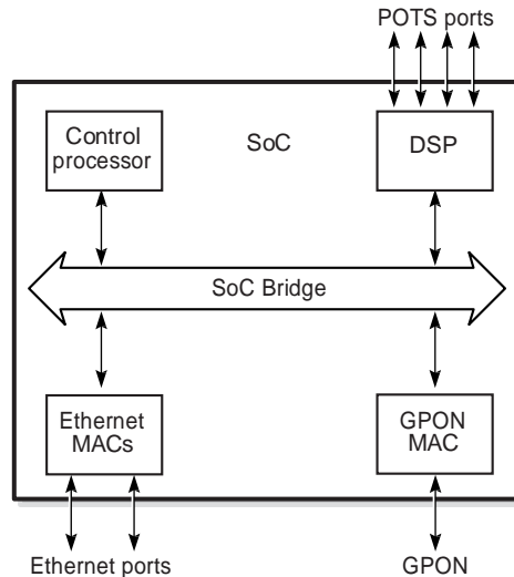
Figure 18 G-240W-F ONT hardware block
