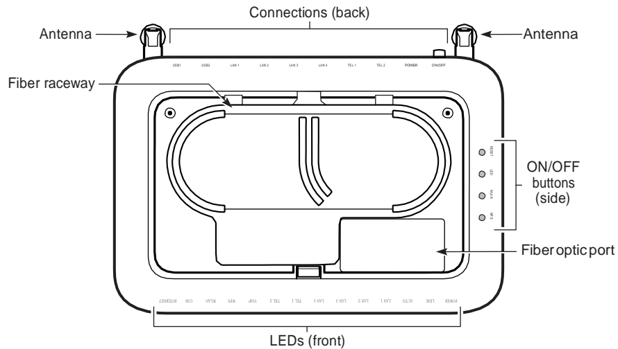
Figure 27 G-240W-F indoor ONT fiber optic port (bottom view)
