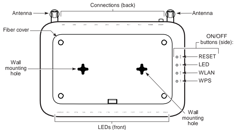
Figure 25 G-240W-F indoor ONT Reset, LED, WLAN, and WPS buttons (side)
