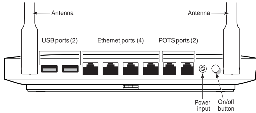
Figure 26 G-240W-F indoor ONT connections (back view)
