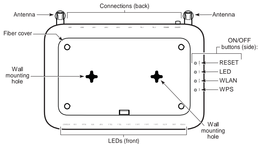
Figure 21 G-240W-F indoor ONT wall mounting holes (bottom view)
