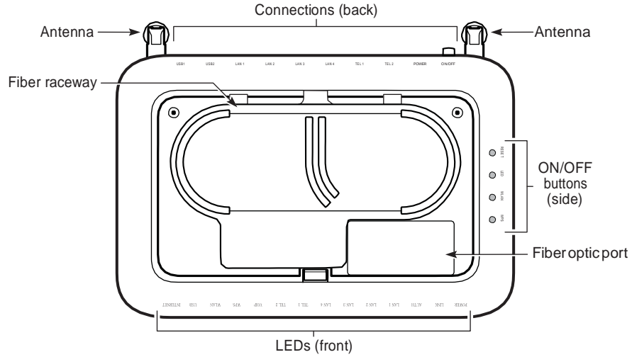
Figure 15 G-240W-F ONT Reset, LED, WLAN, and WPS buttons and fiber optic connection (bottom and side view)
