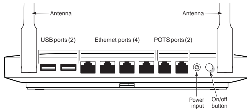
Figure 14 G-240W-F indoor ONT physical connections (back view)
