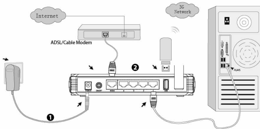
Figure 2-1 Hardware Installation of the PW-3G401/PW-3G401D 3G Wireless Lite-N Router
