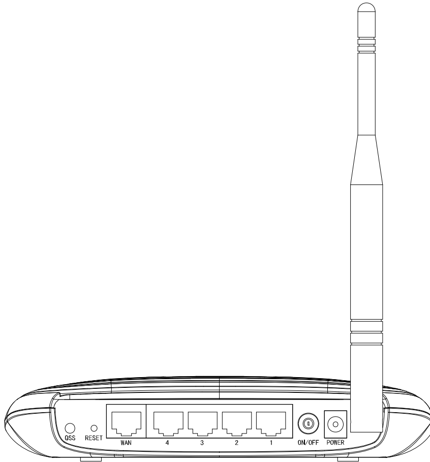
Figure 1-2 Rear Panel sketch
