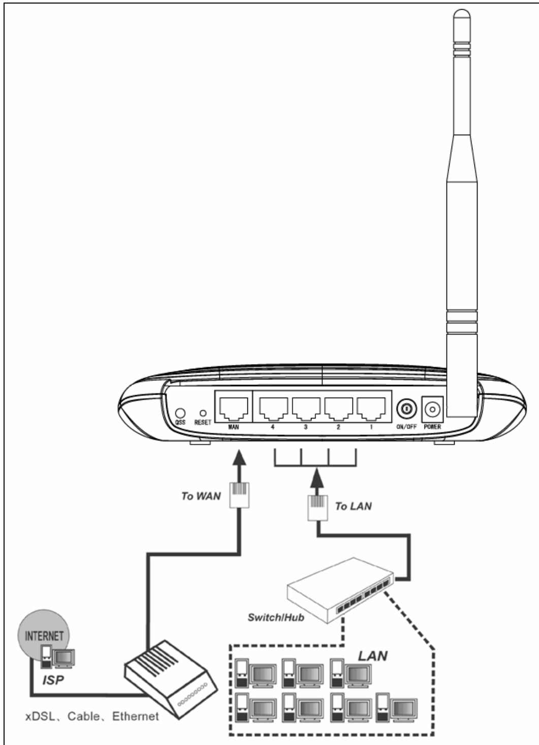
Figure 2-1 Hardware Installation of the TL-WR741ND 150Mbps Wireless N Router
