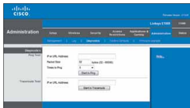
Administration > Diagnostics
