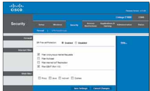
Security > Firewall
