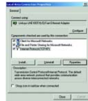
Figure 5-4: TCP/IP
