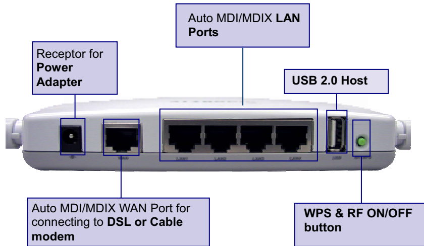
Figure 1: Router's Side Panel
