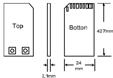
Figure 1 SX-SDWAG Dimensions
