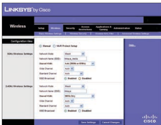
Wireless &gt; Basic Wireless Settings
