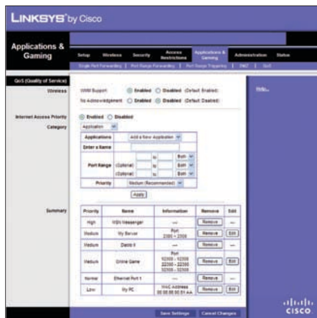
Add a New Application
