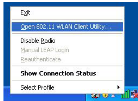
Client Utility
